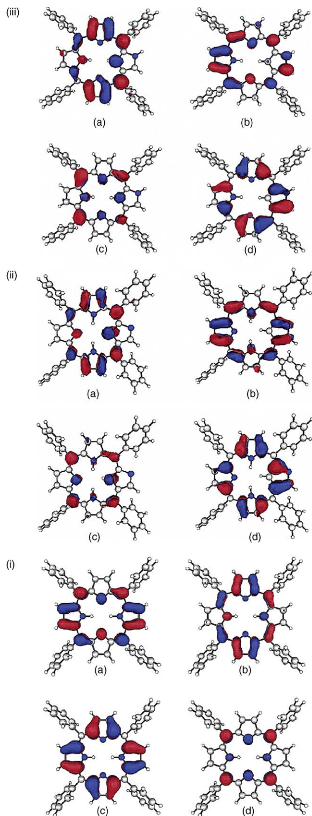
Fig. 7. Plots of the LUMO + 1 (a), LUMO (b), HOMO (c), and HOMO-1 (d) molecular orbitals for H 2 TTP (i), internally protonated H 2 NCTTP (ii), and externally protonated H 2 NCTTP (iii). These orbitals were calculated at the B3LYP/6-31G (d) level [37].
